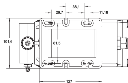
Kynar Head Shown, dimensions in mm
